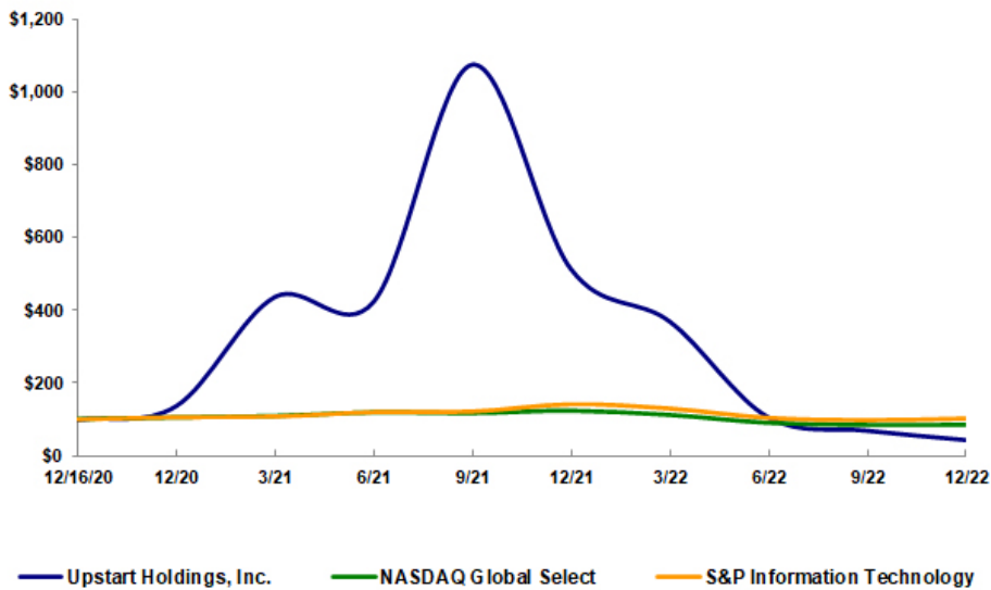
COMPARISON OF 25 MONTH CUMULATIVE TOTAL RETURN* Among Upstart Holdings, Inc., the NASDAQ Global Select Index and the S&P Information Technology Index
